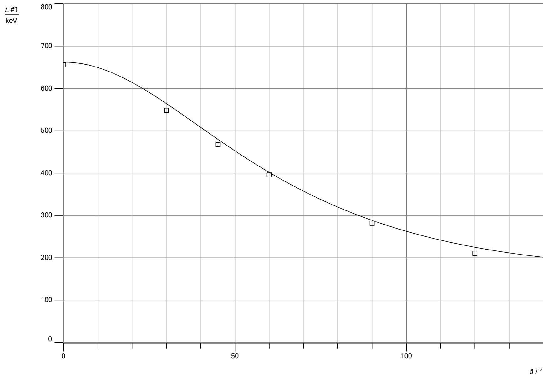
Evaluation - Target - Brass (Data with evaluation and fitting) - CASSY Lab 2
